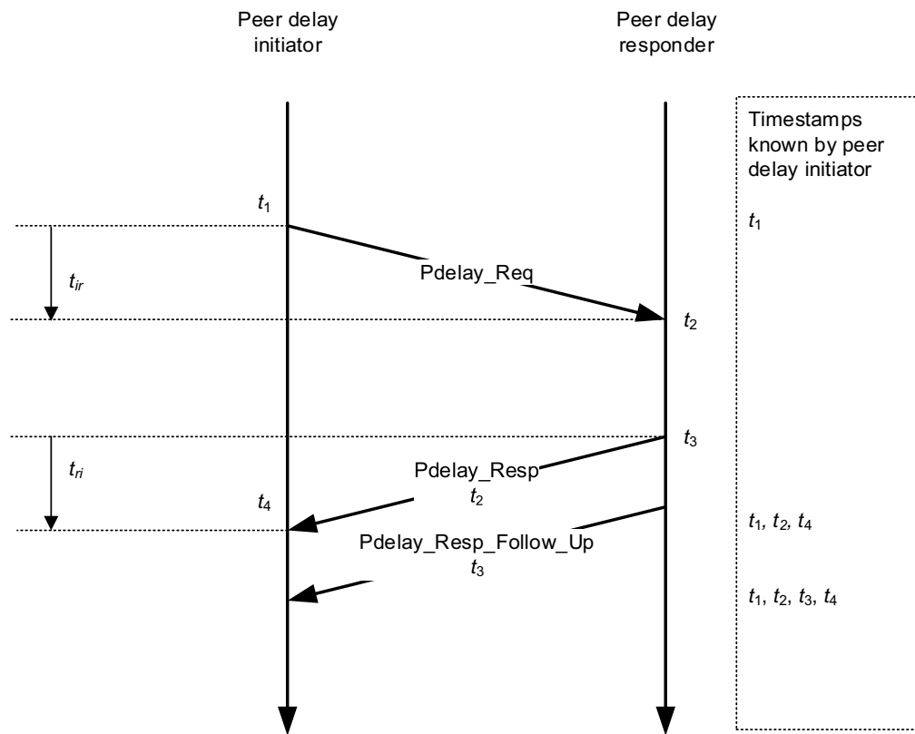
Figure 11-1—Propagation delay measurement using peer-to-peer delay mechanism
